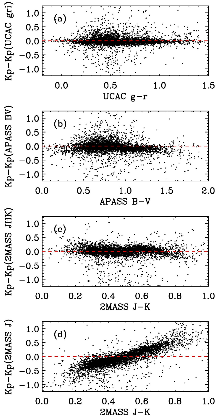
Figure 1: A comparison of original Kepler magnitude ( K_p ) values from the Kepler Input Catalog (Brown et al. 2011) to Kepler magnitudes calculated from UCAC gri (panel a), APASS BV (panel b), 2MASS JHK (panel c), and 2MASS J (panel d) as a function of color, based on a random sample of 5000 stars in the original Kepler field.
