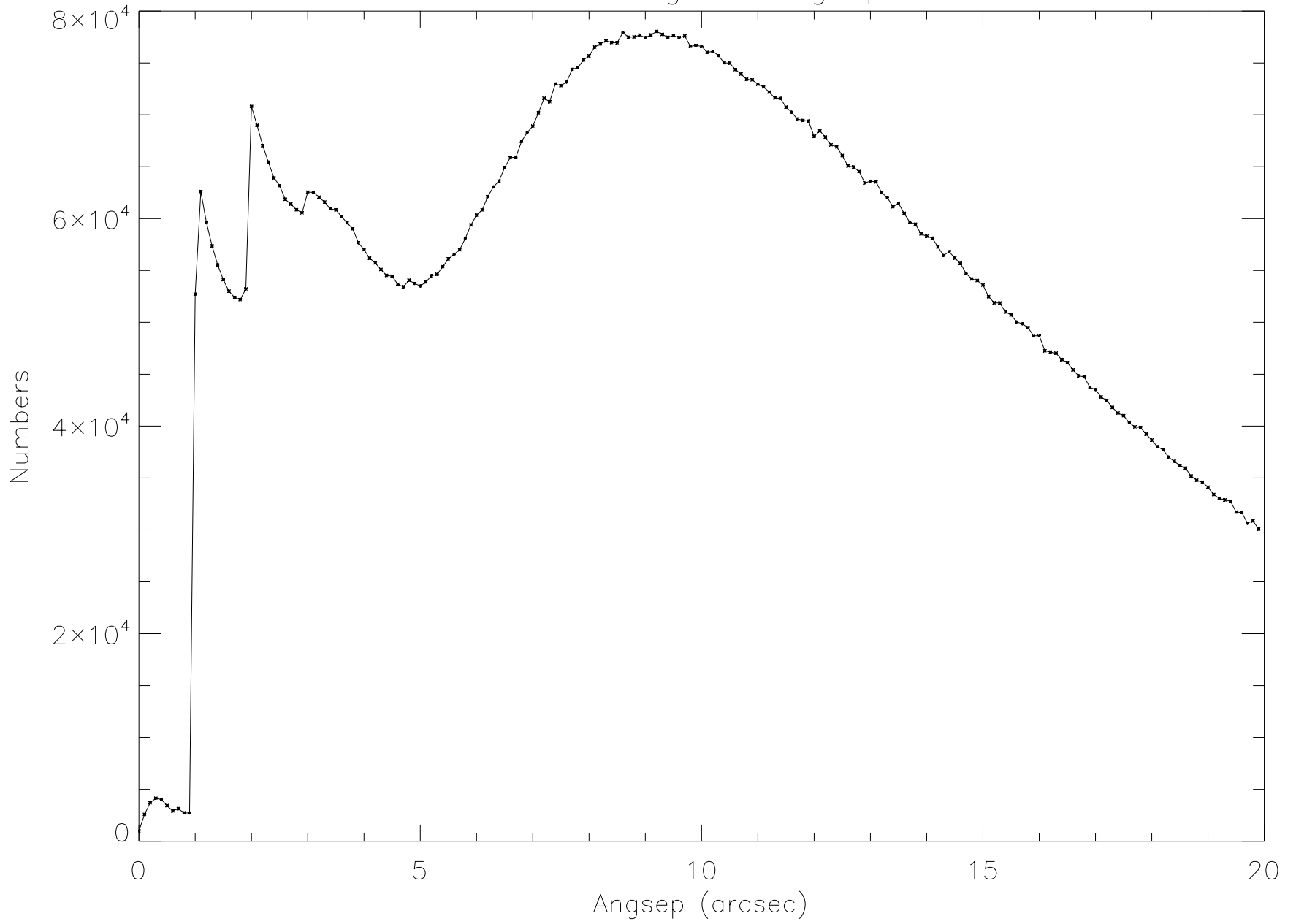
KIC Xmatchings vs angsep dist
