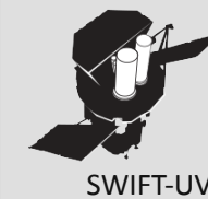
SWIFT-UVOT
